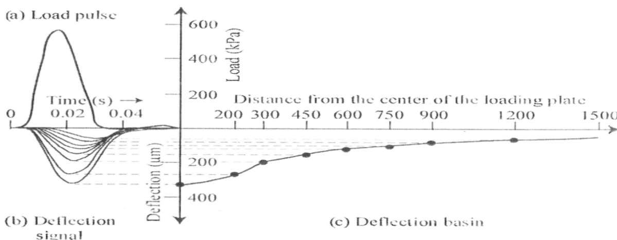
Figure 1: FWD Loading and Pavement Response (Doré & Zubeck, 2009)
